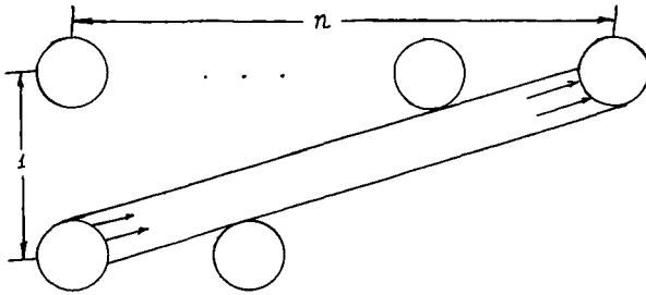
Fig. 2. The outgoing vectors form the cell A_n .
