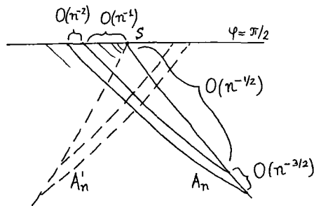
Fig. 1. A supersingular point S and a cell A_n near it.
