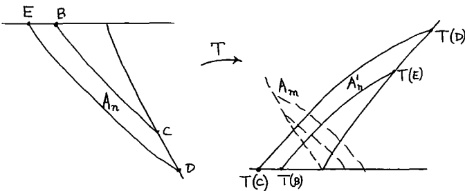
Fig. 3. The image of A_n under the map T is a reverse cell, A'_n .
